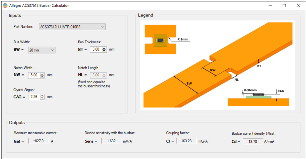
Figure 22: ACS37610 Busbar Calculator GUI
