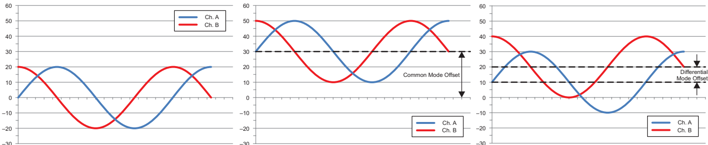
Figure 6 Left: No Offset, Middle: Common Mode Offset; Right: Differential Mode Offset
