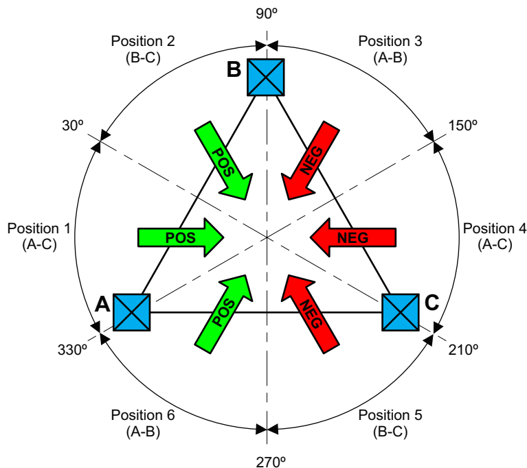
Figure 17: Mounting Positions
