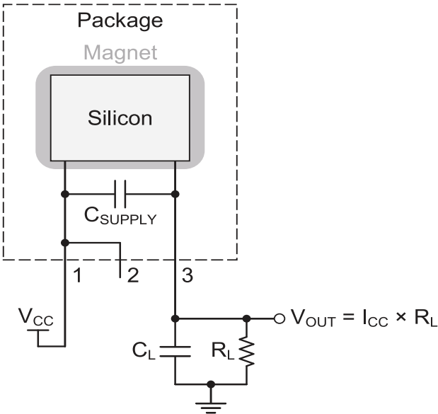
Figure 3: Typical Application Circuit
