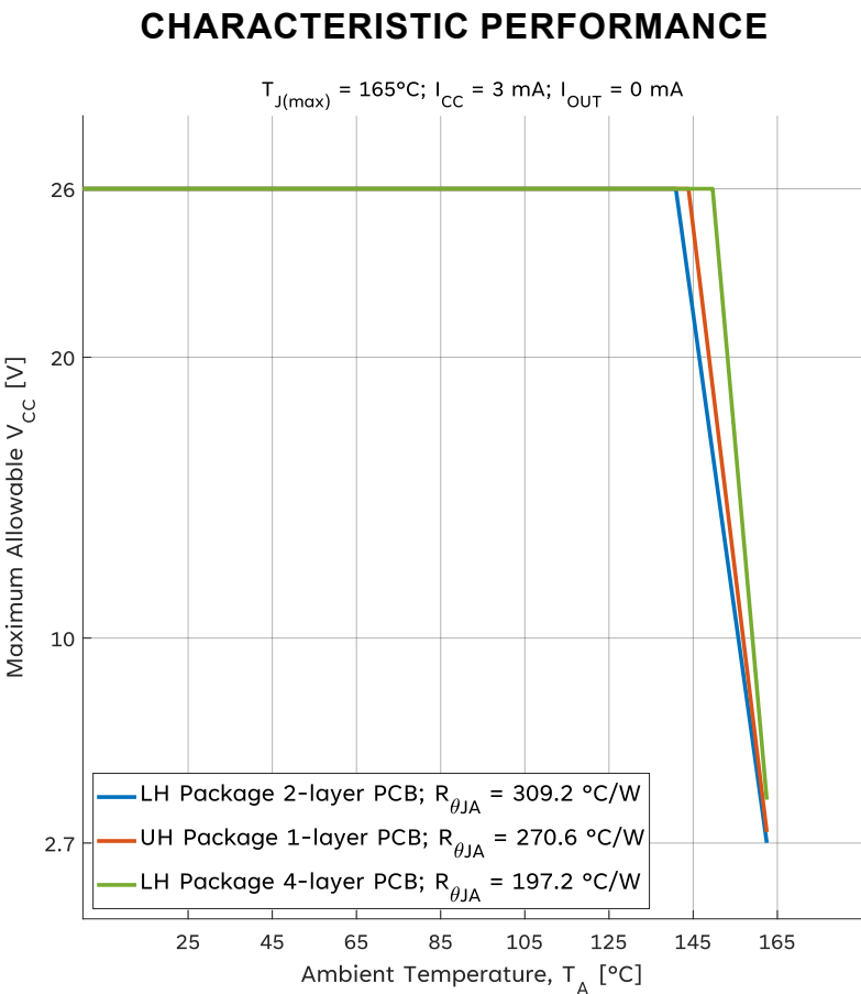
Figure 6: Power Derating
