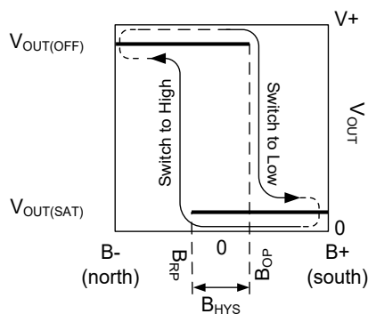
Figure 5: Hall Latch Output State vs. Magnetic Field
