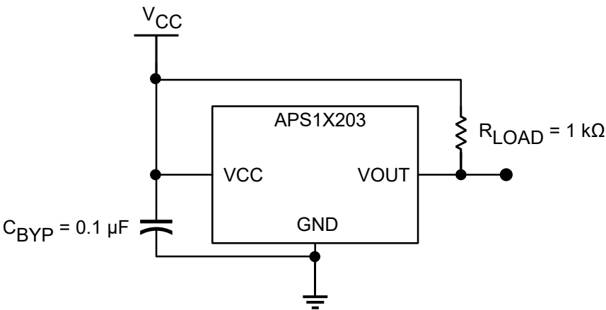
Figure 4: Typical Application Circuit
