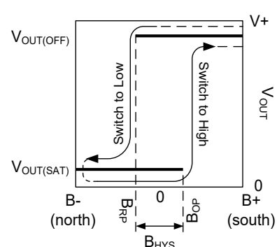
Figure 5: Hall Latch Output State vs. Magnetic Field
