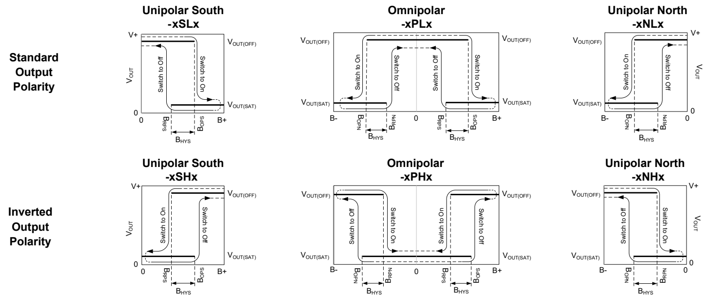
Figure 5: Hall Switch Output State vs. Magnetic Field
