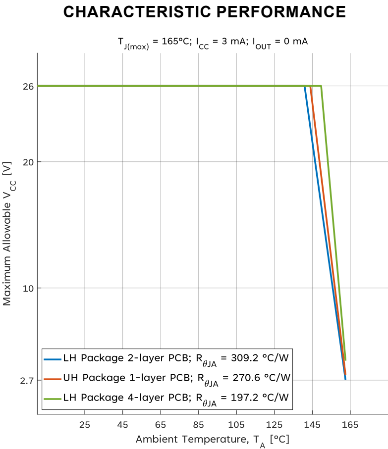
Figure 6: Power Derating
