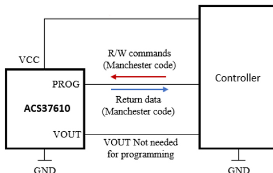
Figure 7: Programming Connections—Mode 2
