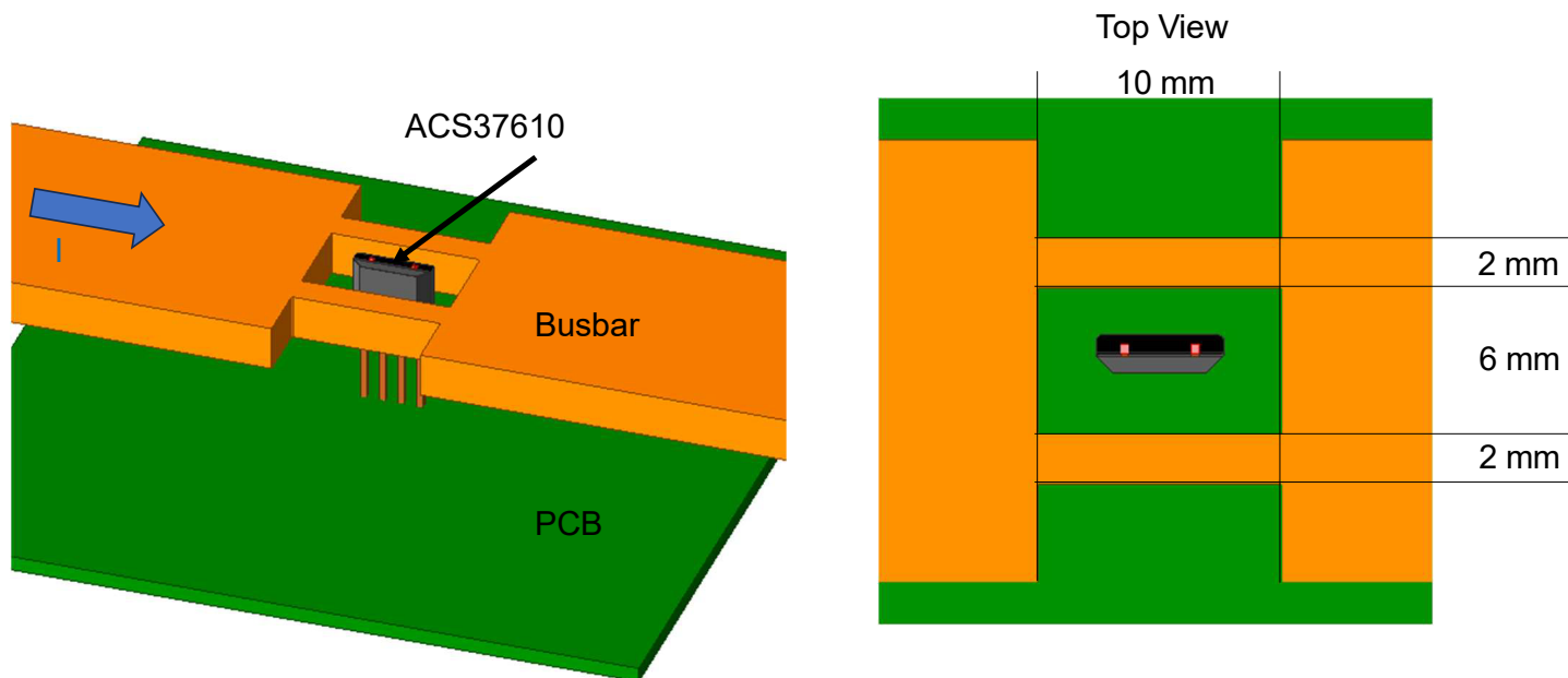
Figure 33: Busbar Current-Sensing Application—Reference Busbar Design with Dual Bridge
