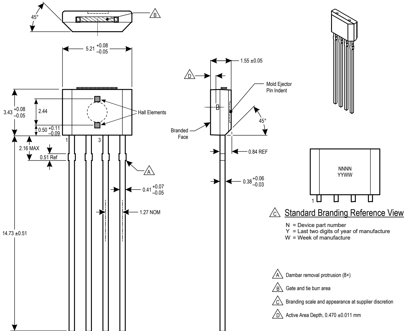
Figure 37: Package OK, 4-Pin SIP, TN Leadform (Straight Leads)
