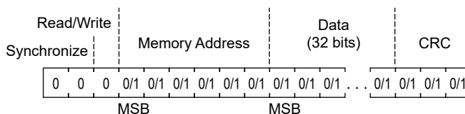
Figure 11: Write Sequence
