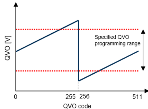
Figure 25: QVO Trim Range
