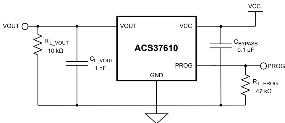
Figure 1: Typical Application Circuit (Programming Pin Used)
