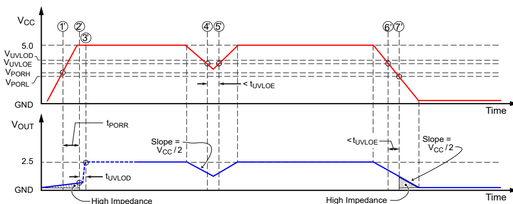
Figure 32: POR and UVLO Operation, Fast Rise Time Case
