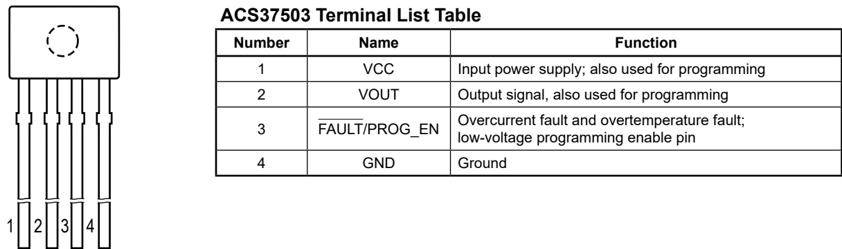
Figure 2: KT Package Pinout Diagram (Ejector pin mark on opposite side)
