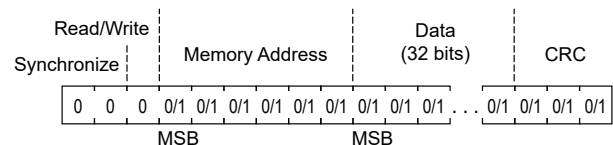
Figure 20: Write Sequence
