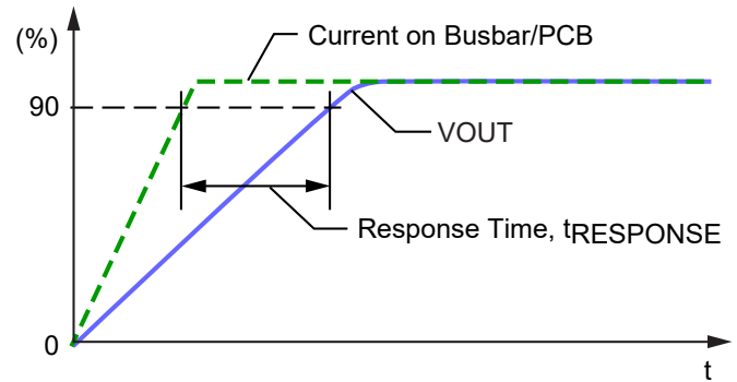
Figure 6: Response time
