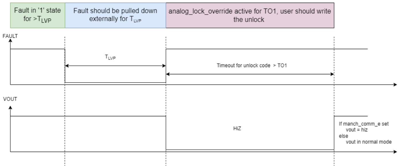
Figure 16: Low-Voltage Runtime Unlock Timing Diagram
