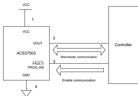
Figure 14: Low Voltage Programming Connection
