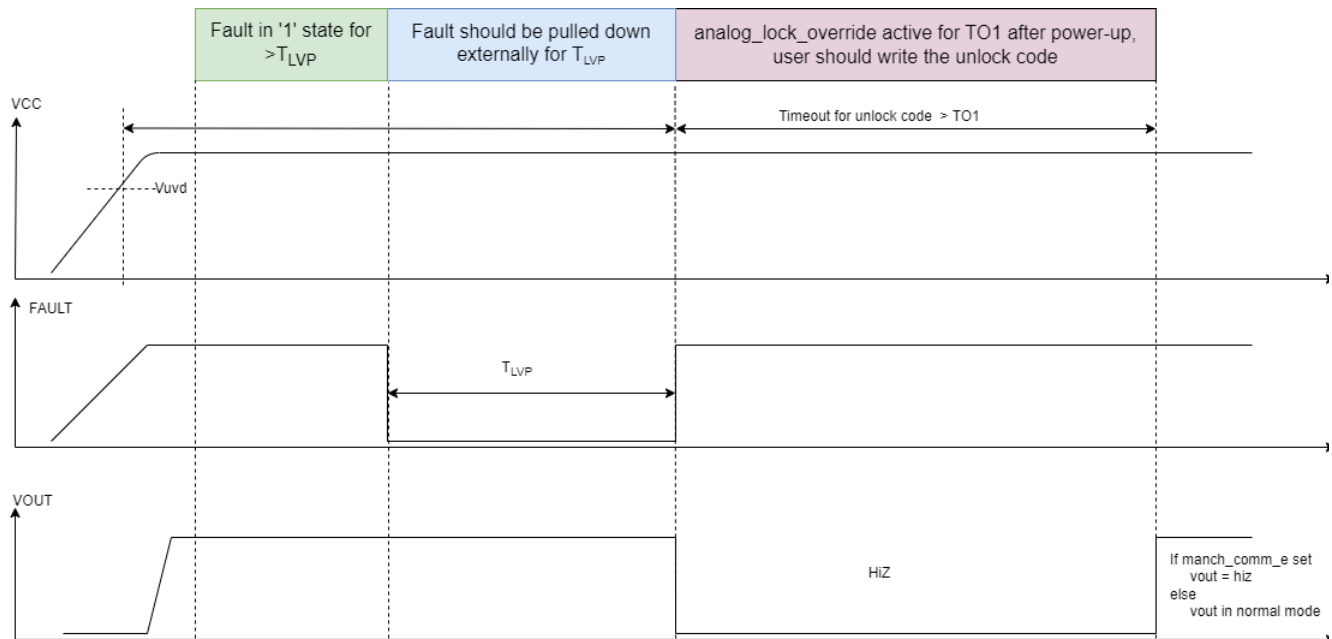
Figure 15: Low-Voltage Startup Unlock Timing Diagram
