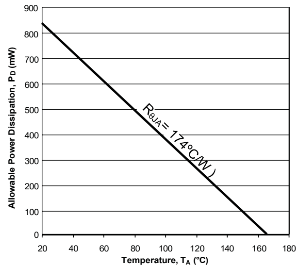
Allowable Power Dissipation versus Ambient Temperature
