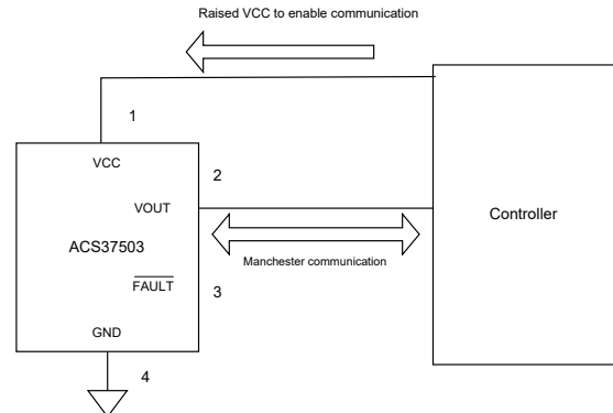
Figure 13: Programming Connection Using OVD
