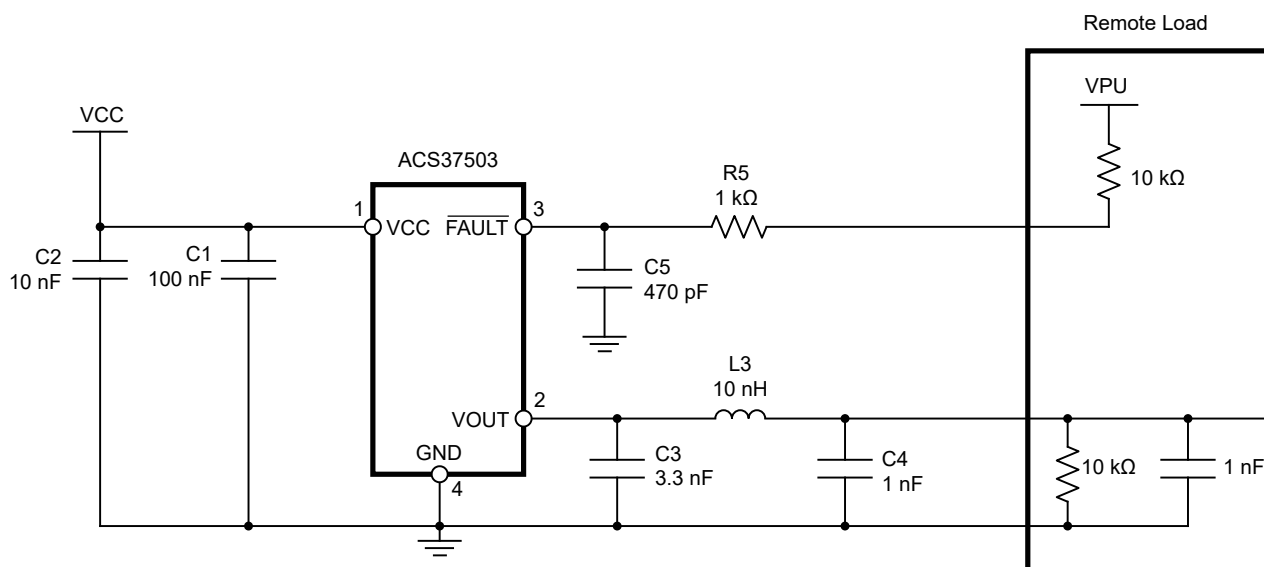
Figure 4: Circuit for EMC-critical applications
