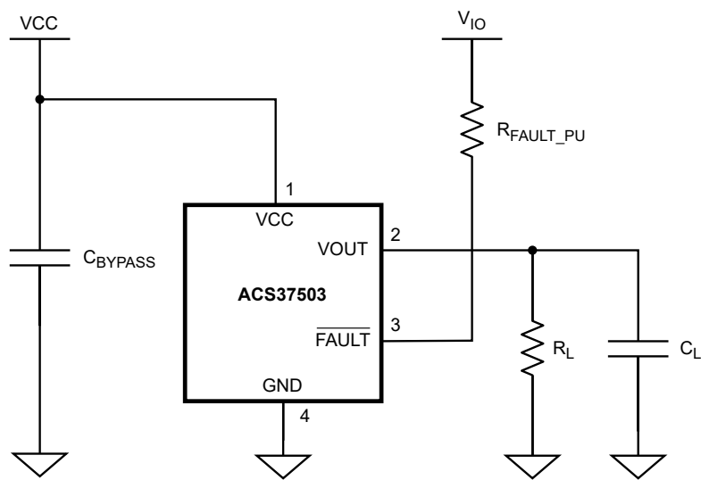
Figure 3: Typical Application Drawing
