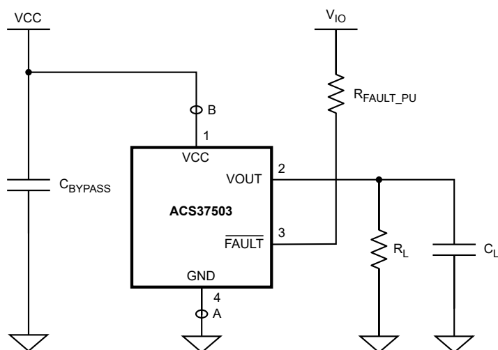
Figure 8: Connection for Detecting Broken Wire
