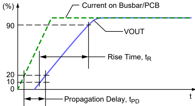
Figure 5: Propagation delay and rise time
