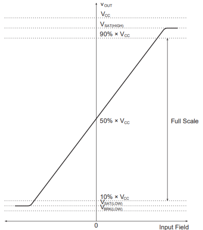
Figure 7: VOUT Characteristics of ratiometric device
