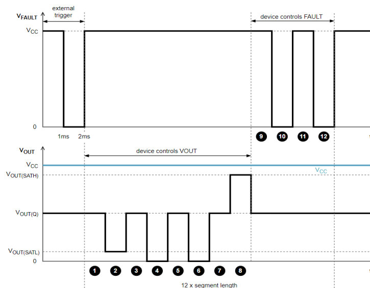
Figure 12: Output Test Sequence
