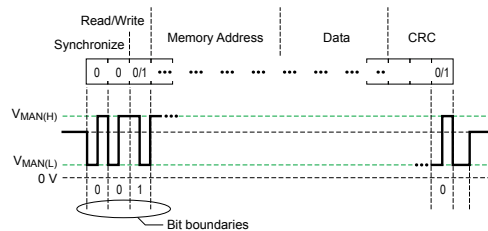
Figure 17: General Format For Serial Interface Commands
