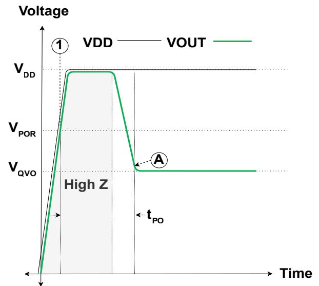
Figure 7: Power-On Delay, t_{PO}
