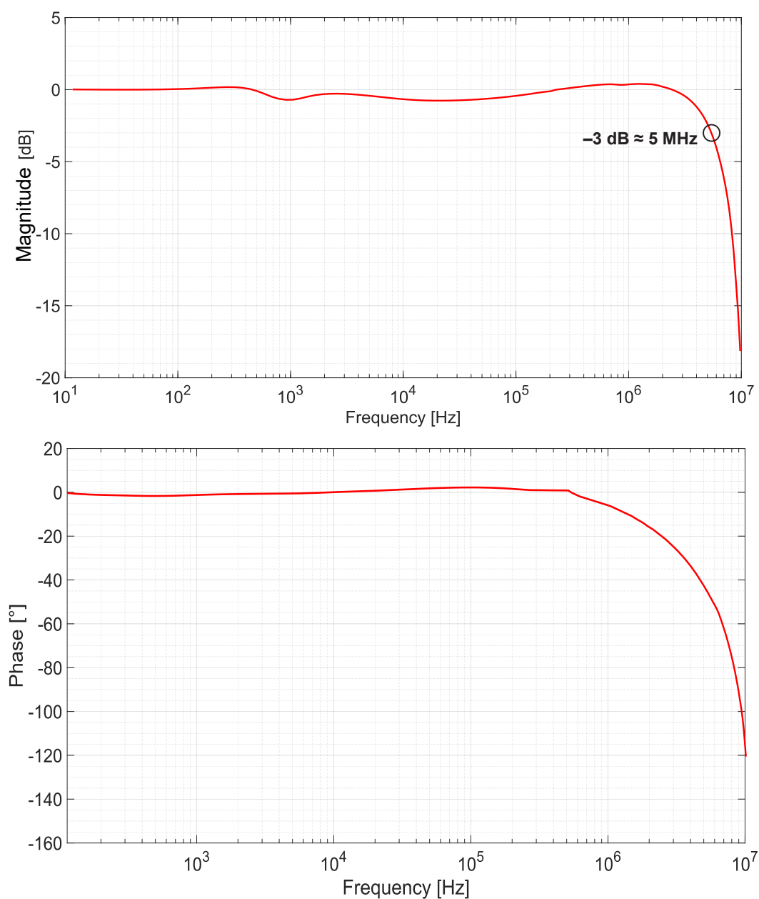
Figure 4: Typical Frequency Response
