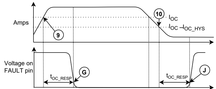
Figure 9: Fault Timing Diagram
