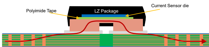
Figure 11: No Vias Under Copper Pads, LZ Package
