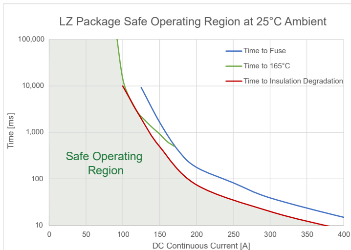
Figure 15: LZ Package Safe Operating Region
