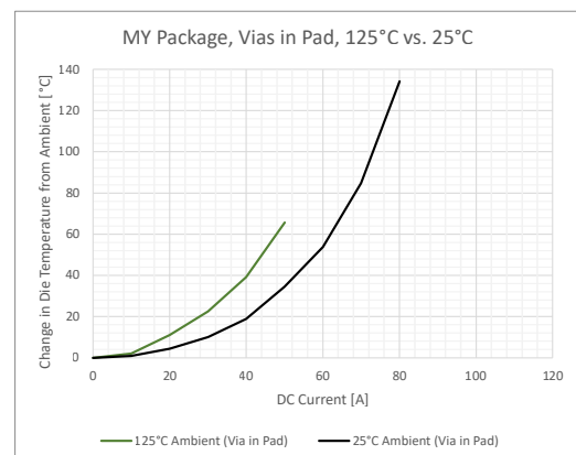
Figure 14: MY Package Comparison at 125°C and 25°C, In-Pad Vias
