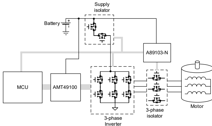
Figure 35: Alternative Independent Drive System
