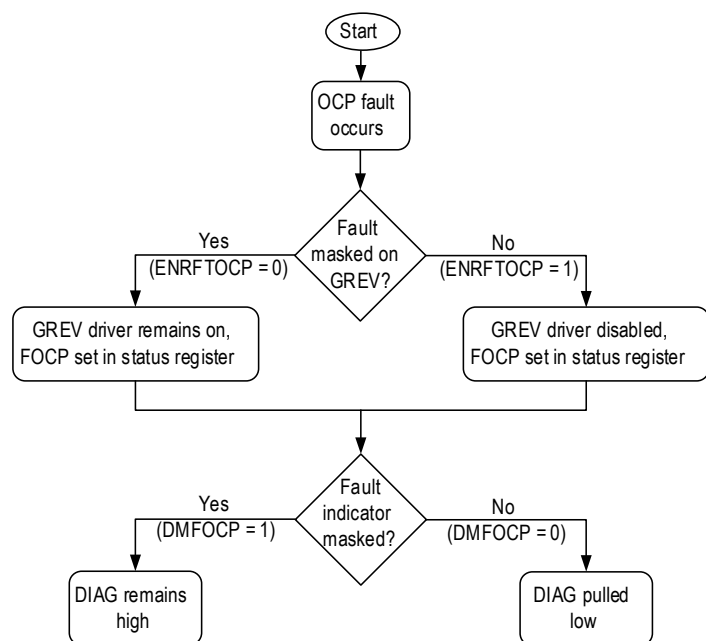
Figure 31: Fault-Masking Flowchart
