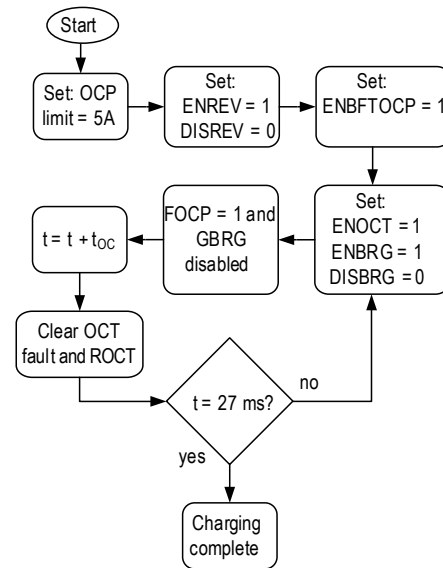
Figure 30: Flowchart for Charging DC Link Capacitor
