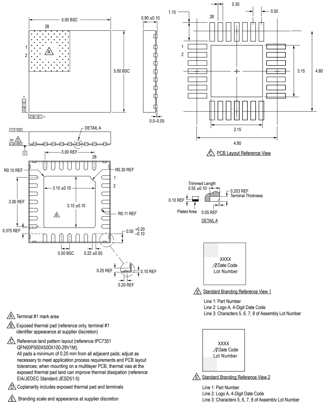
Figure 46: Package ET, 28-Contact QFN with Exposed Pad and Wettable Flank
