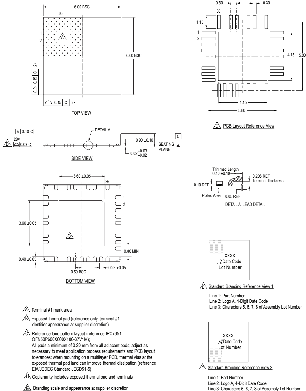
Figure 45: Package EV, 28-Contact QFN with Exposed Pad and Wettable Flank
