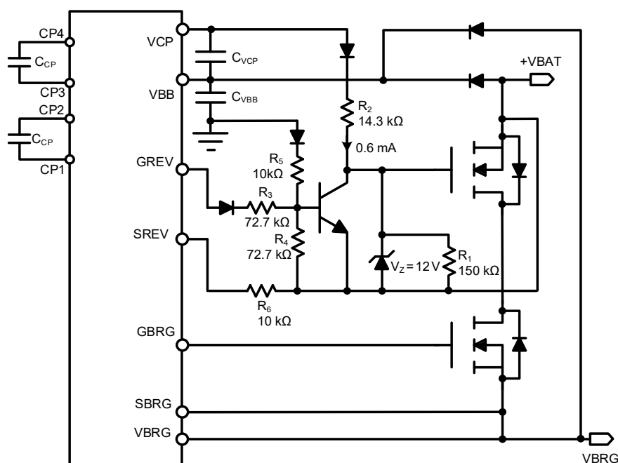
Figure 44: Recommended Circuit
