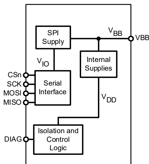
Figure 11: A89103-N Internal Regulators
