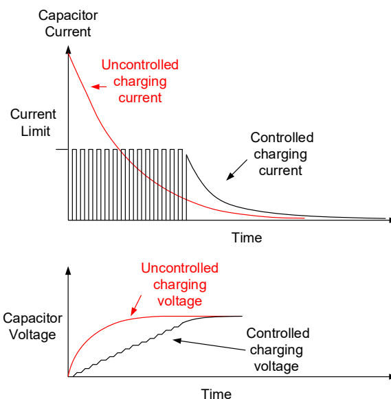
Figure 28: Controlled Capacitor Charging Current and Voltage
