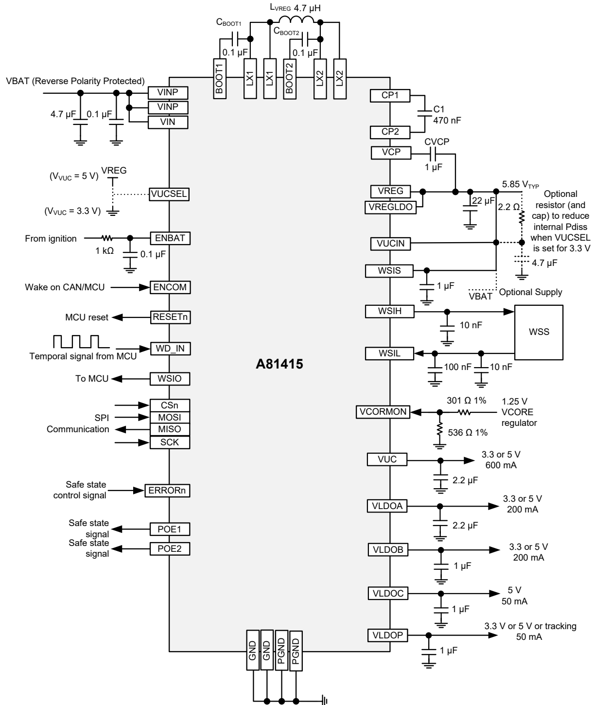
Figure 3: Application Schematic
