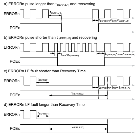
Figure 17: POEx response to toggling ERRORn signal
