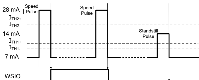
Figure 37: Standstill Pulse with Mode 3
