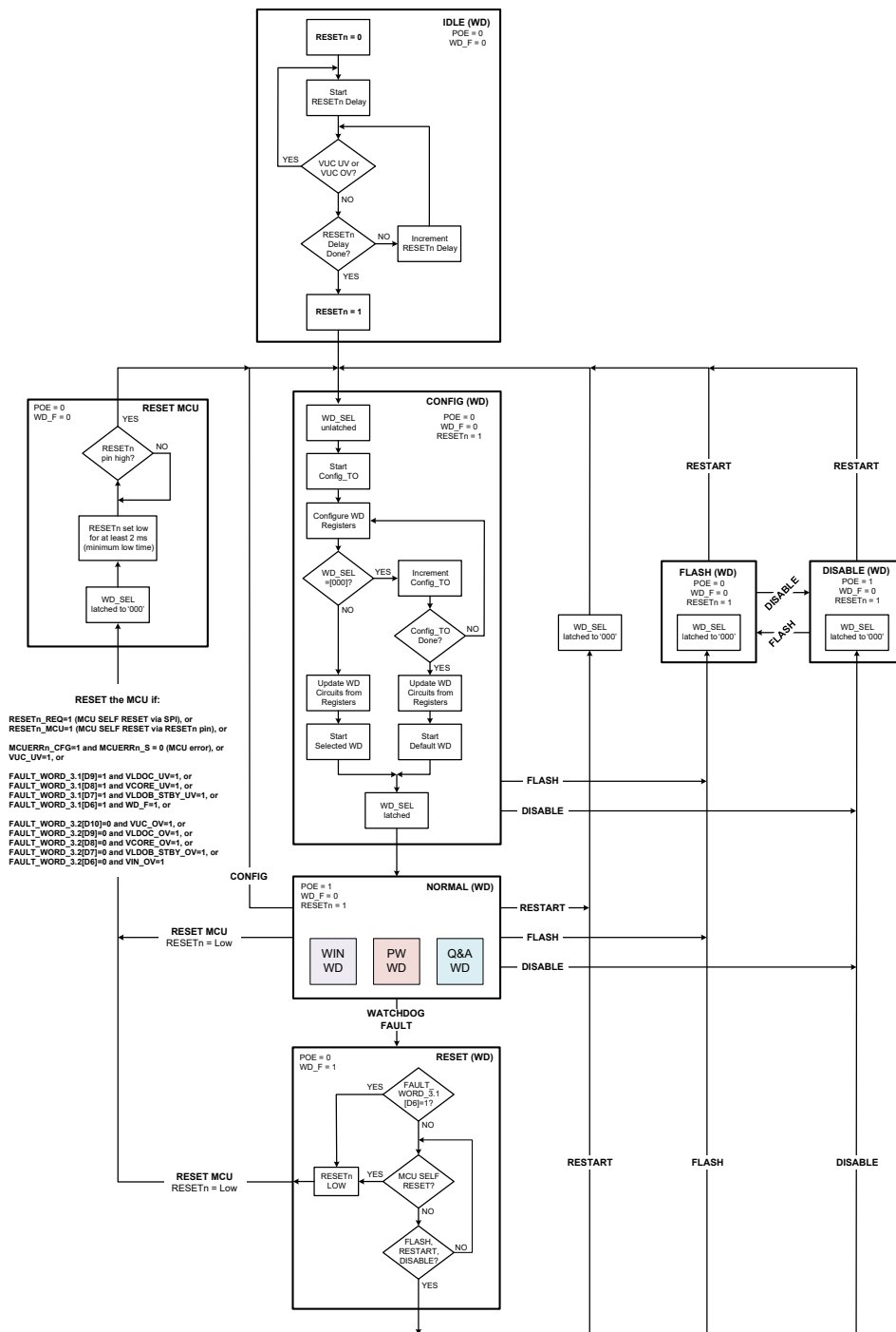
Figure 29: State Diagram of Watchdog Operation
