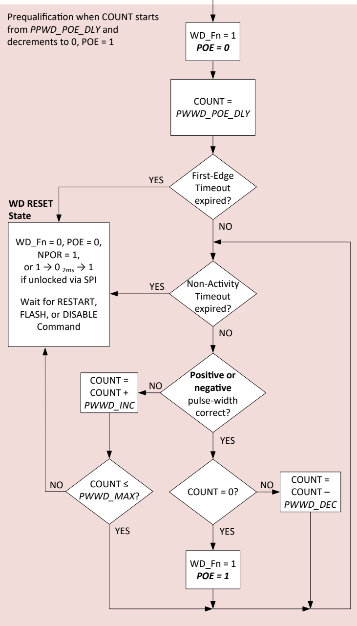
Figure 30: WWD and PWWD Flow Charts
