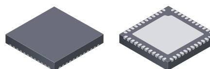
48-pin QFN (suffix EV) 7 mm × 7 mm with exposed pad and wettable flank Not to scale
