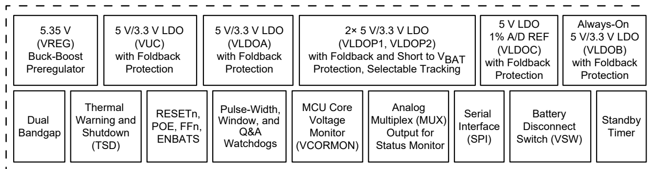
Figure 1: A81412 Simplified Block Diagram
