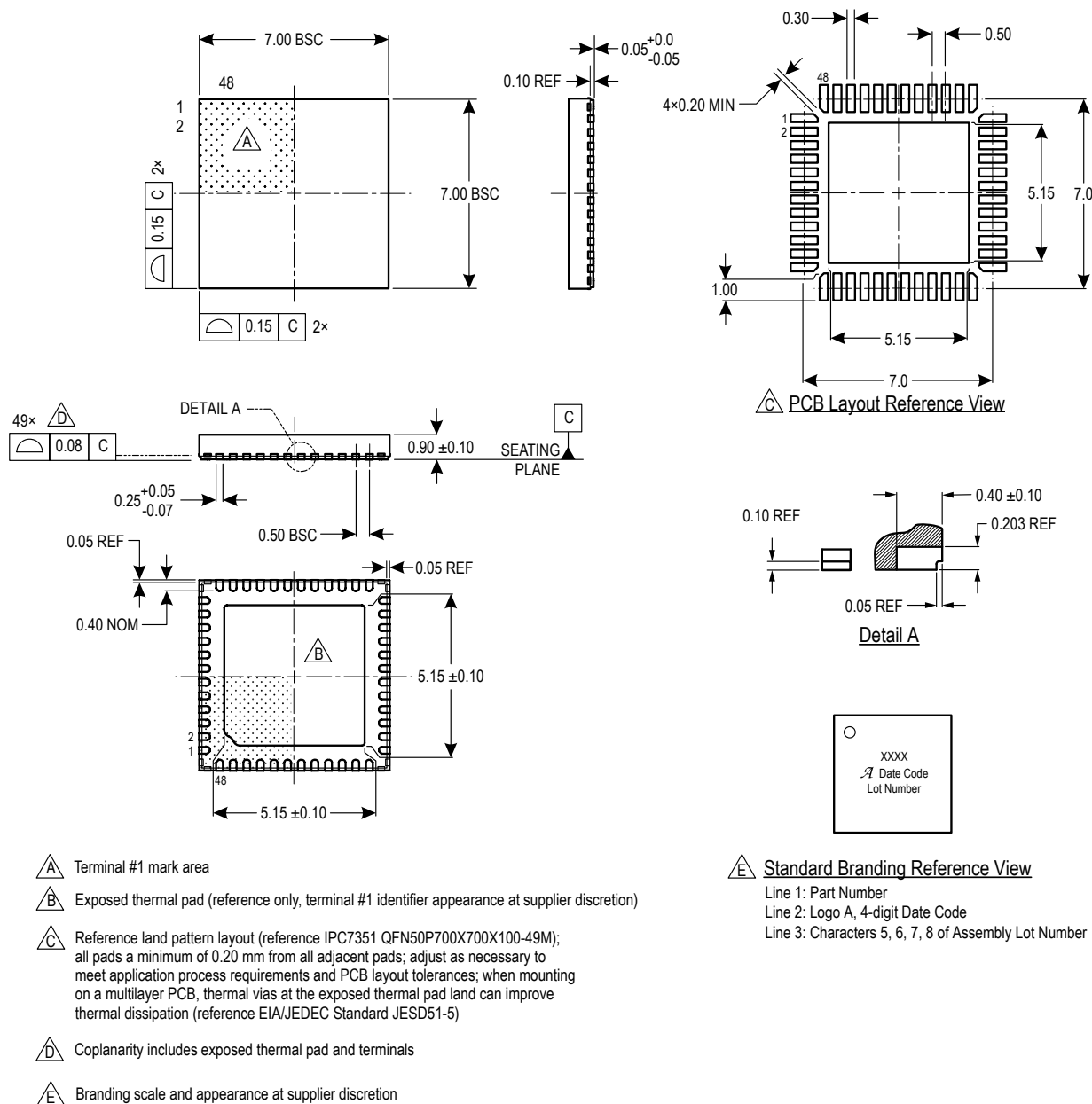
Figure 25: Package EV, 48-Pin QFN with exposed pad and wettable flank
