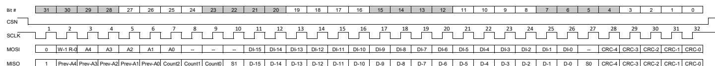
Figure 23: 32-Bit SPI Frame
