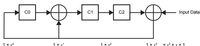
Figure 34: Manchester CRC Calculation
