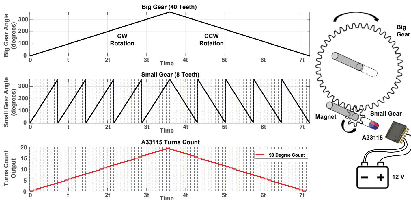
Figure 17: Turns Count Example Application
