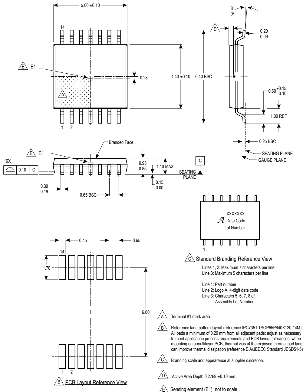
Figure 35: Package LE, 14-Pin TSSOP
