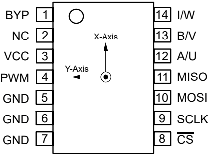
LE 14-Pin TSSOP Pinout Diagram and Axis Definition
