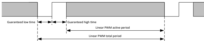
Figure 3: PWM Period
