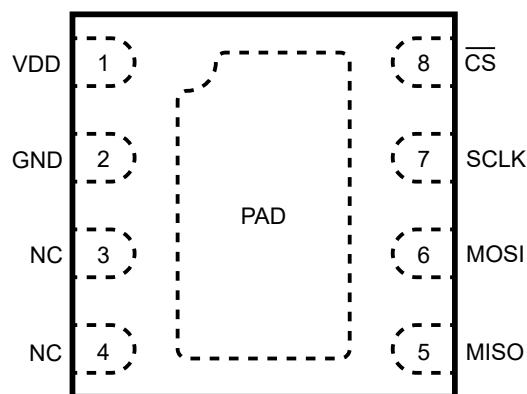
Figure 3: Pinout Diagram (Top of Package)
