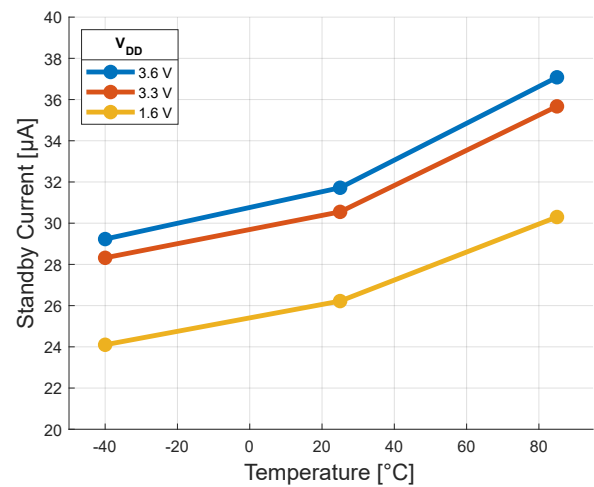
Figure 14: Standby Current
