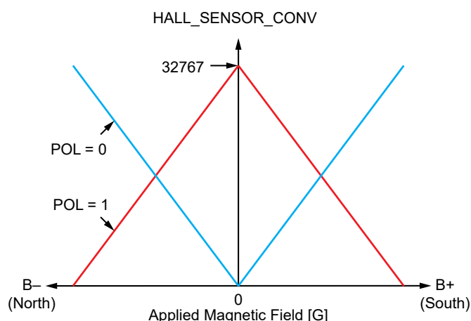
Figure 23: Omnipolar Mode
