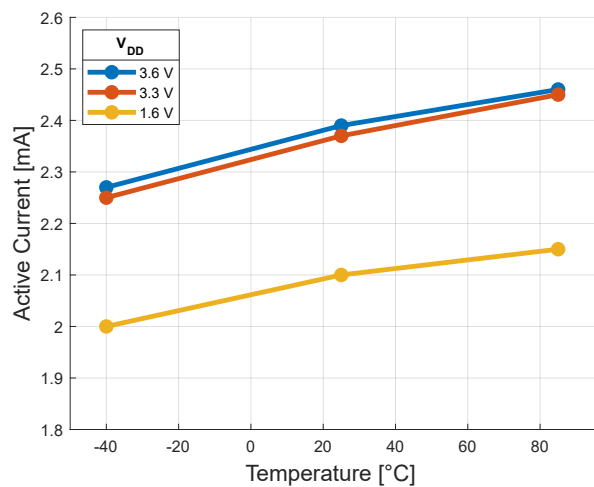
Figure 12: Active Current (-Z Option)
