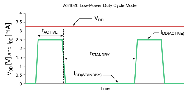
Figure 19: I_{DD} in Low-Power Duty Cycle Mode
