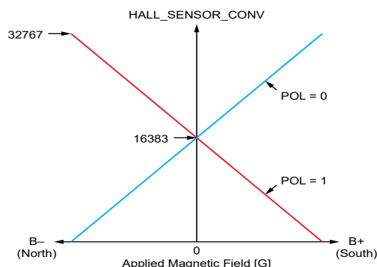
Figure 20: Bipolar Mode with 50% Offset
