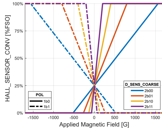
Figure 7: Bipolar Output with 25% Offset (OFFSET_COARSE = 2b00)
