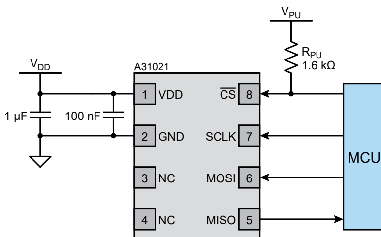
Figure 4: Typical Application Circuit
