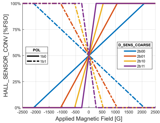
Figure 6: Bipolar Output with 50% Offset (OFFSET_COARSE = 2b01 or 2b10)
