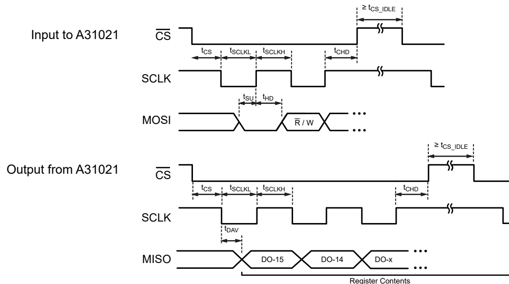
Figure 5: SPI Interface Timing Diagram
