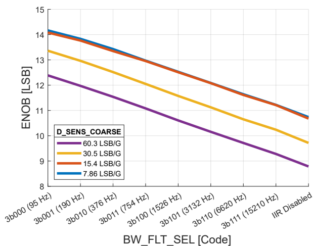
Figure 18: Effective Number of Bits (ENOB) (-Z Option)
