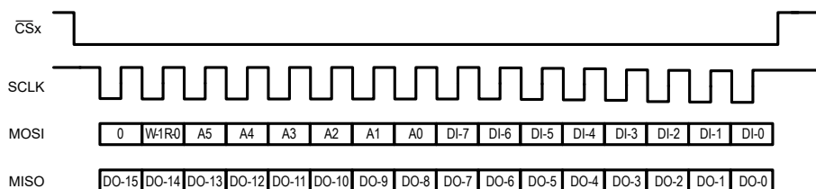
Figure 24: SPI Frame
