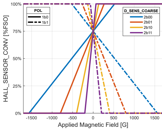
Figure 8: Bipolar Output with 75% Offset (OFFSET_COARSE = 2b11)
