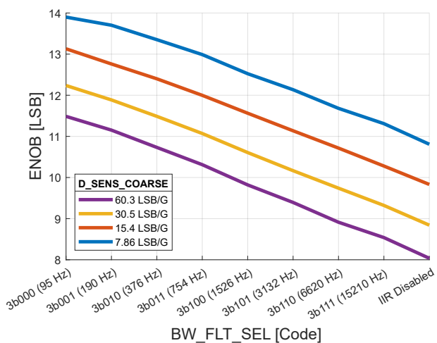
Figure 17: Effective Number of Bits (ENOB) (-X Option)
