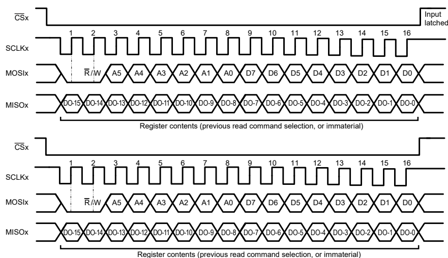
Figure 26: SPI Read Timing Diagram
