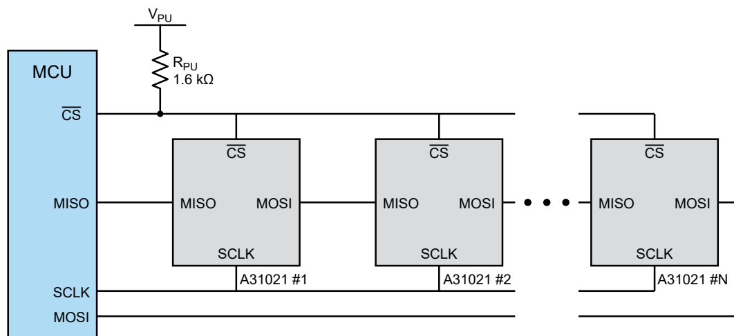
Figure 27: RSDO Application Diagram
