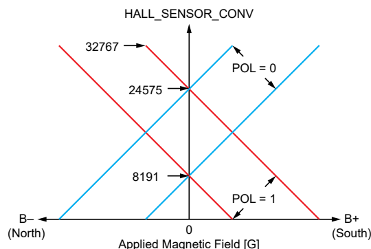
Figure 21: Bipolar Mode with 25% and 75% Offset
