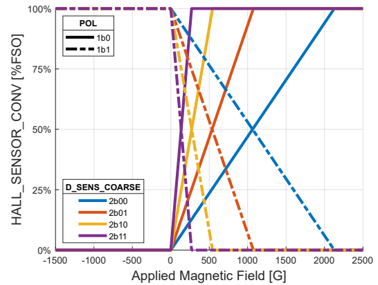
Figure 9: Unipolar South Output
