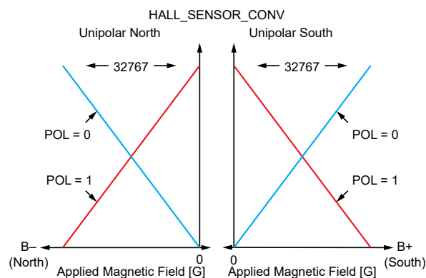
Figure 22: Unipolar North (Left) and Unipolar South (Right)
