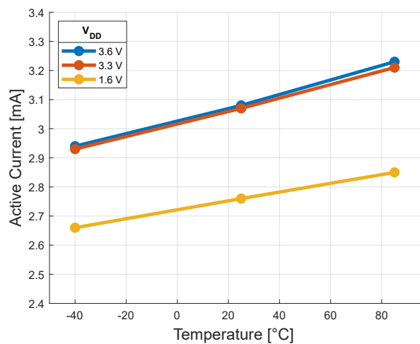
Figure 13: Active Current (-X Option)
