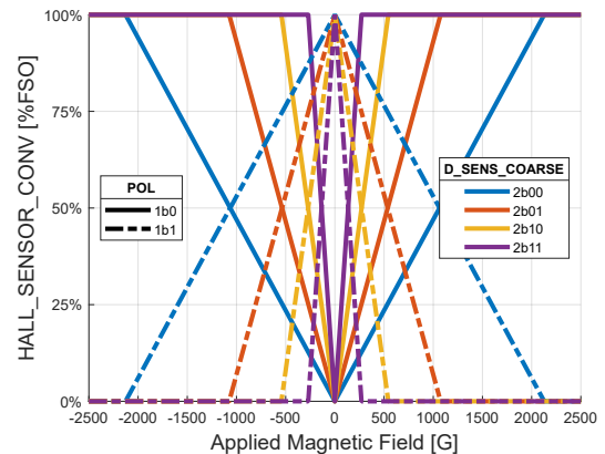
Figure 11: Omnipolar Output
