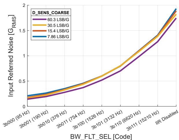
Figure 15: Output Noise Standard Deviation (-X Option)
