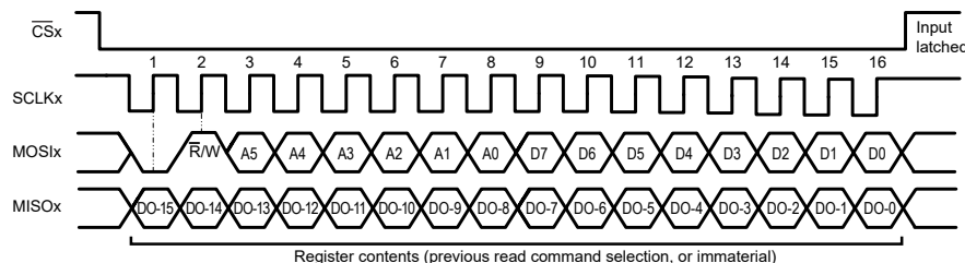
Figure 25: SPI Write Timing Diagram
