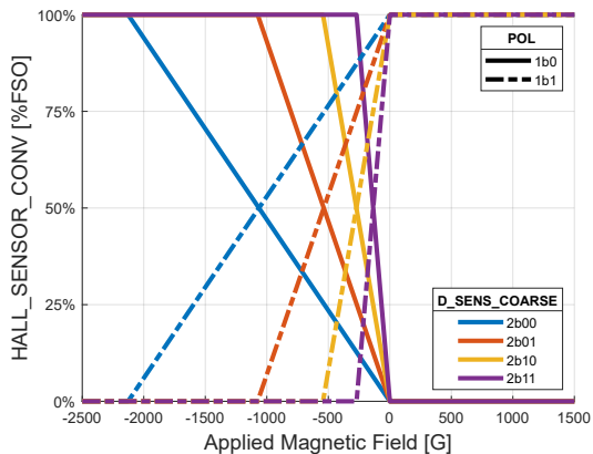
Figure 10: Unipolar North Output
