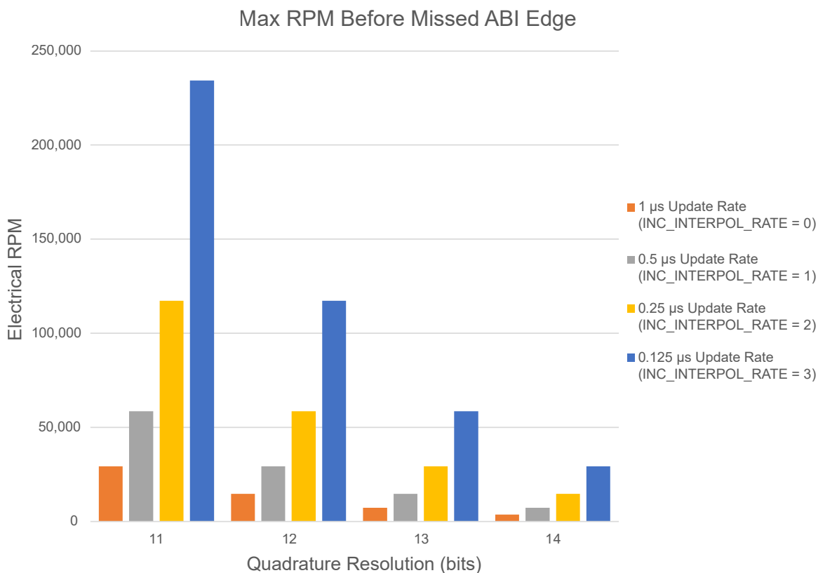
Figure 30: A17803 Resolution Selection for ABI
