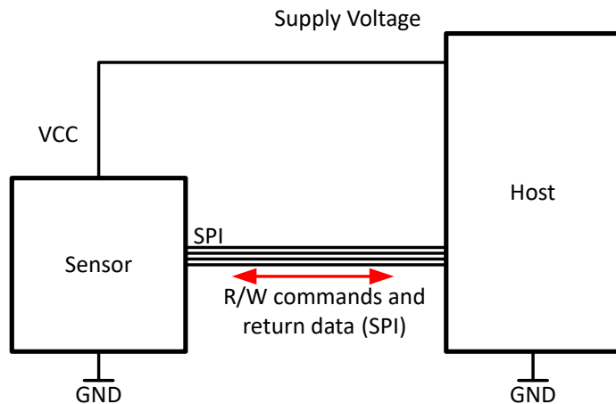
Figure 37: SPI Interface Programming Setup
