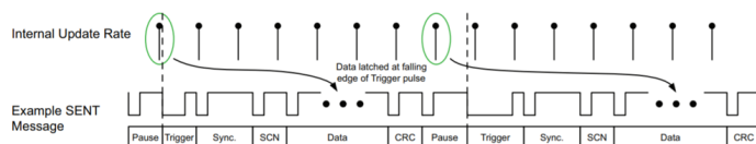
Figure 18: TSENT Data Synchronization and External Trigger Synchronous Mode
