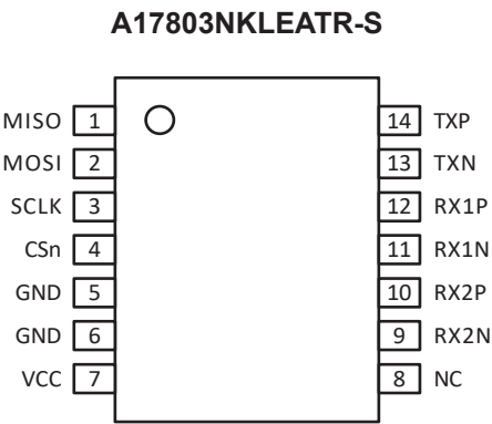
Package LE 14-pin TSSOP Pinout Drawing
