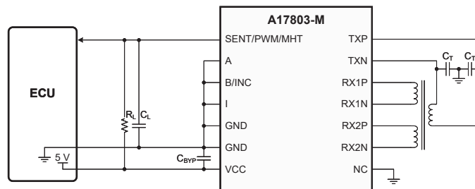
Figure 3: Typical A17803 configuration using SENT or PWM interface
