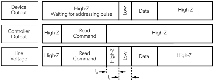
Figure 52: Manchester Read Response Timing
