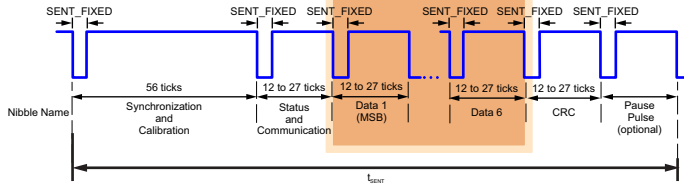
Figure 15: SENT Data Nibble
