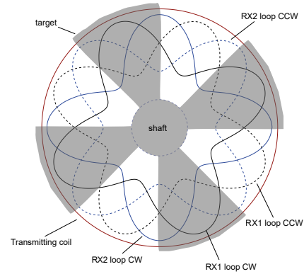
Figure 8: Coil and target design for 4 electrical periods
