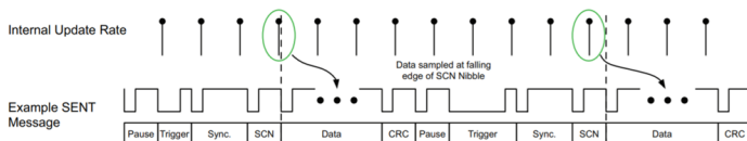
Figure 19: TSENT Data Synchronization and External Trigger Asynchronous Mode
