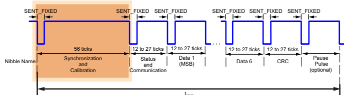
Figure 13: Synchronization and Calibration Pulse in SENT Message
