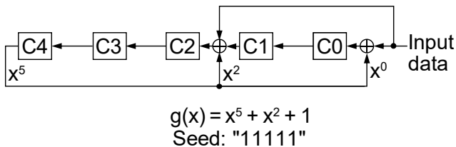
Figure 44: CRC Calculation with Left Shift Register
