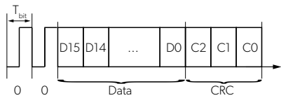
Figure 51: Manchester Read Acknowledge Command
