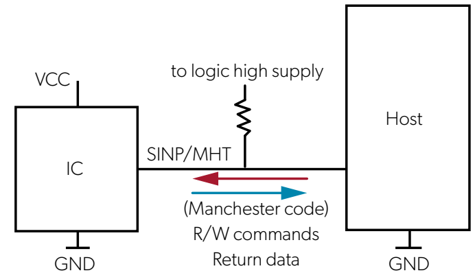
Figure 48: Manchester Programming Interface Setup
