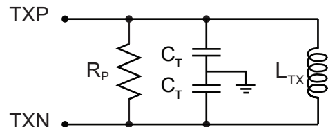
Figure 9: LC tank equivalent circuit. R_p represents losses.
