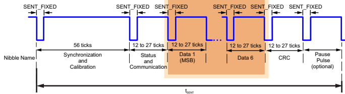
Figure 15: SENT Data Nibble
