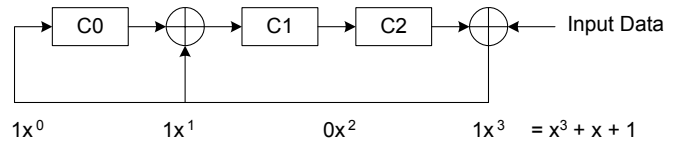
Figure 11: CRC Calculation
