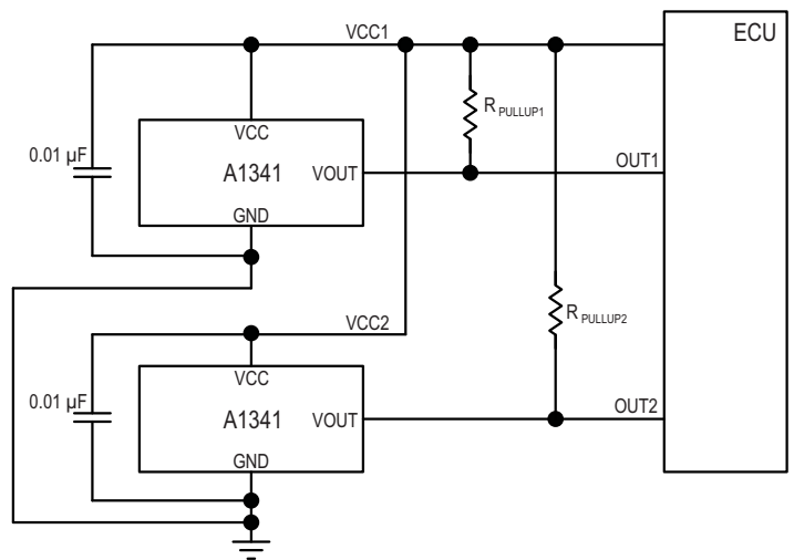
Figure 8: Typical Application
