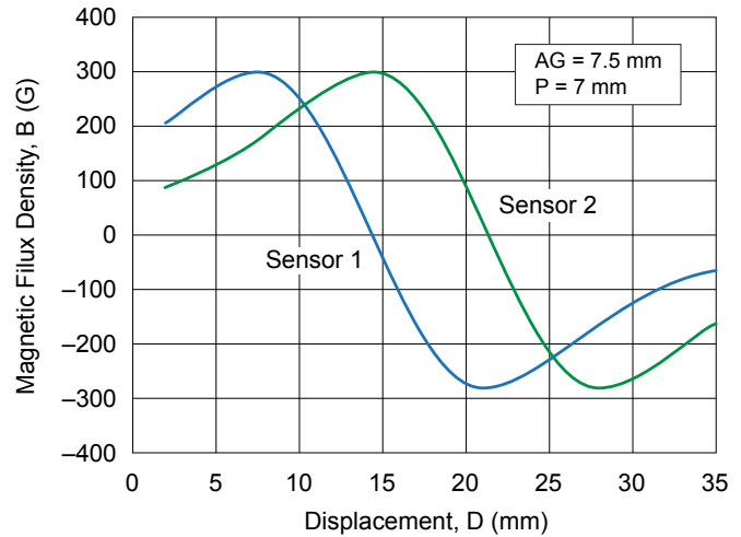
Figure 4. Magnetic flux density versus magnet displacement
