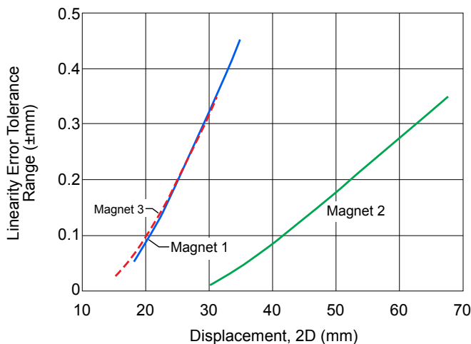
Figure 20. Comparison of linearity error tolerance range ( \pm\text{mm} ) versus absolute displacement, for various magnet configurations
