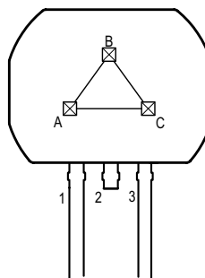
Figure 13: Hall Sensor Configuration
