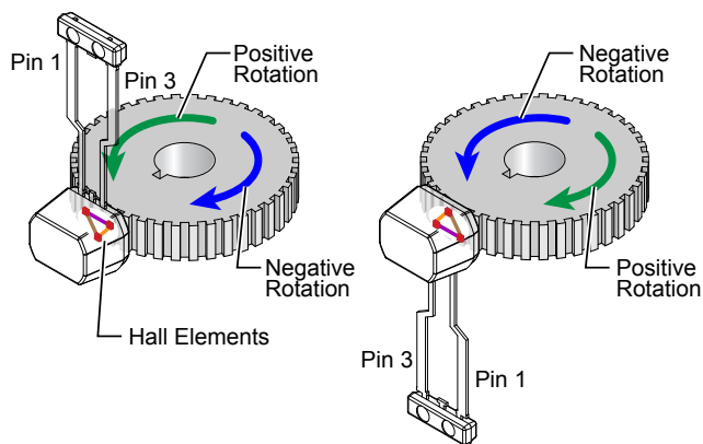
Figure 14: Direction Definition
