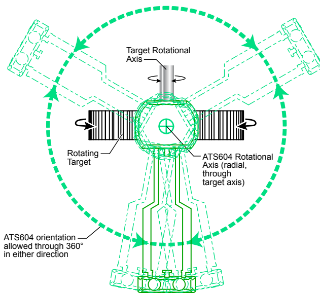
Figure 12: Orientation-Insensitive Mounting
