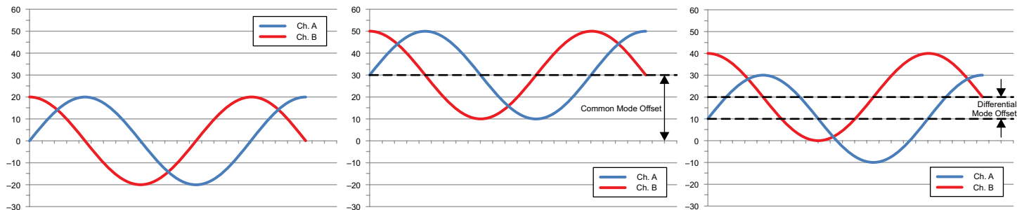
Figure 6 Left: No Offset, Middle: Common Mode Offset; Right: Differential Mode Offset
