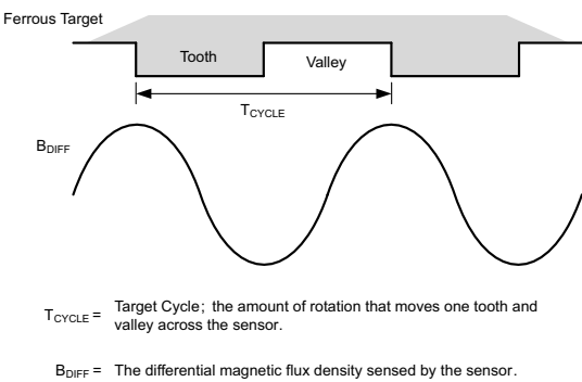
Figure 4: Definition of T_{CYCLE}
