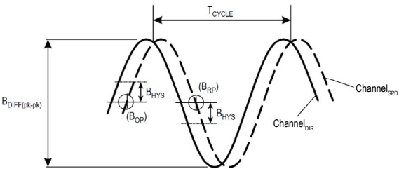
Figure 5: Definition of Switch Point
