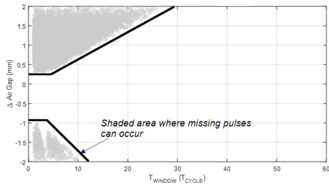
Figure 7: Performance of Differential Sequential Signal Variation
